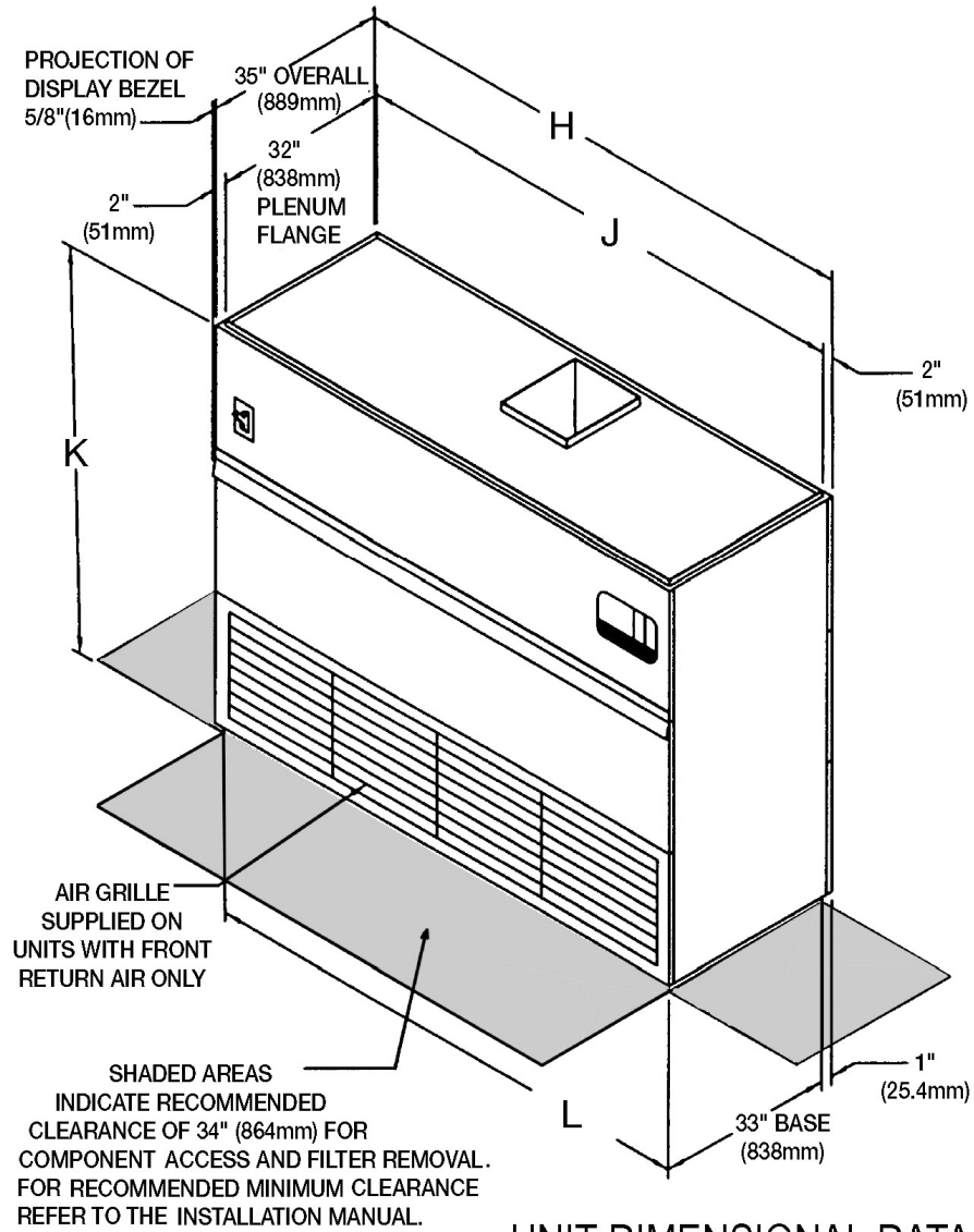
UNIT DIMENSIONAL DATA
