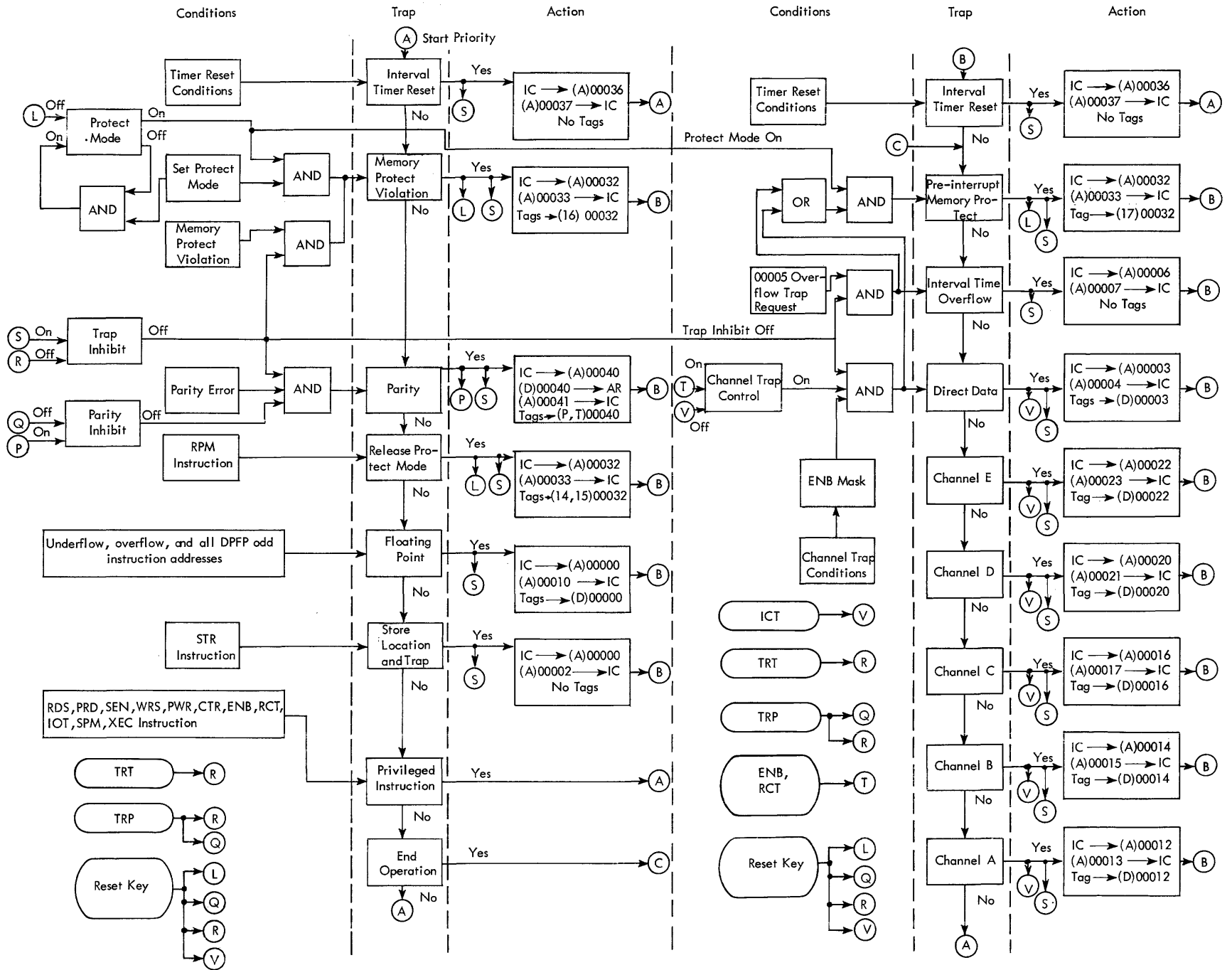
Figure 5. Trap Conditions, Priority, and CPU Action
