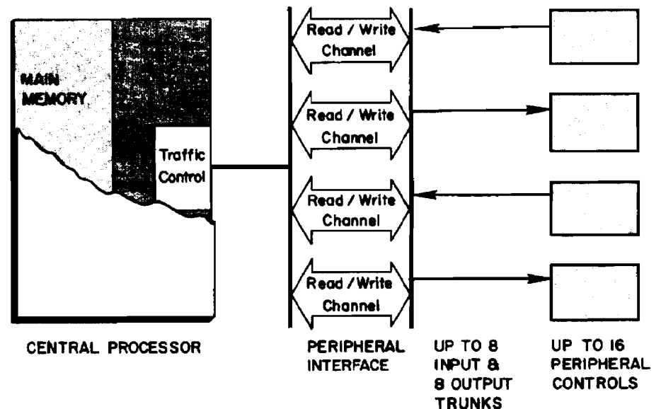
Figure 6. Data Paths Between Central Processor and Peripheral Devices.
