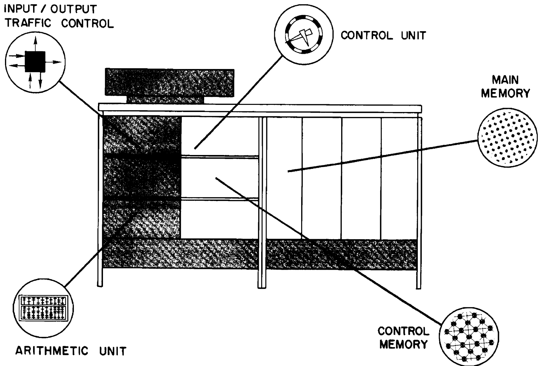
Figure 1. Logical Division of the Central Processor.
