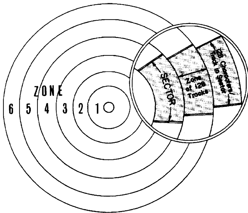
Figure 18. Detail of Disc File Layout.
