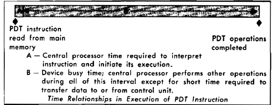
Time Relationships in Execution of PDT Instruction
