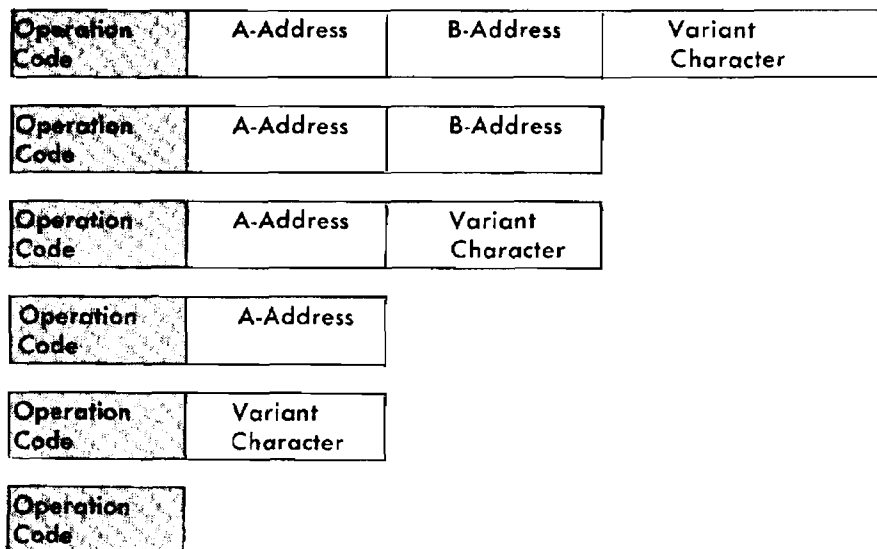
Figure 4. Instruction Formats.
