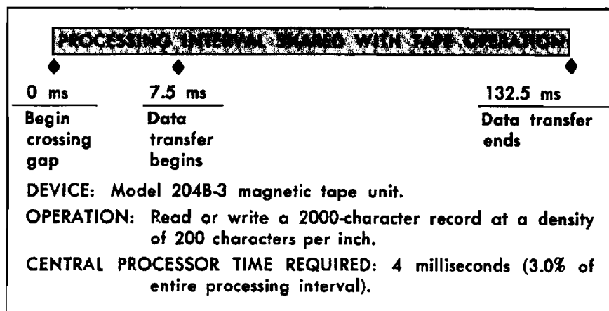
Figure 14. Simultaneity in Typical Tape Operation.
