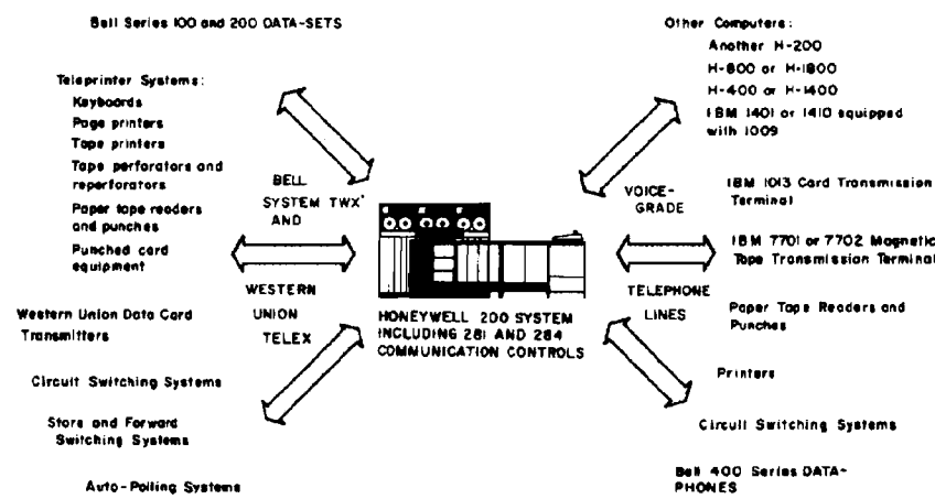
Figure 20. Sample of Possible H-200 Data Communication Connections
