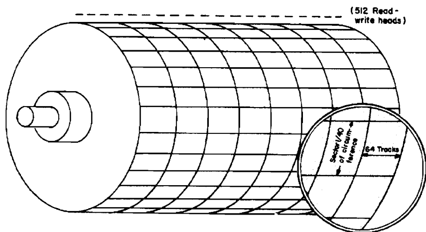
Figure 16. Layout of Drum File Surface.
