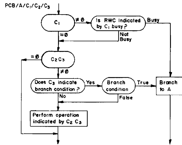
Peripheral Control and Branch Operation
