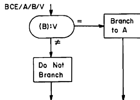
Branch if Character Equal Operation
